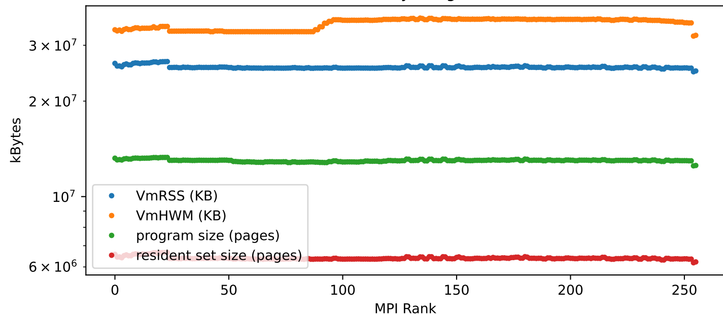
Memory Usage
