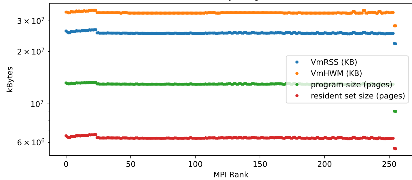
Memory Usage
