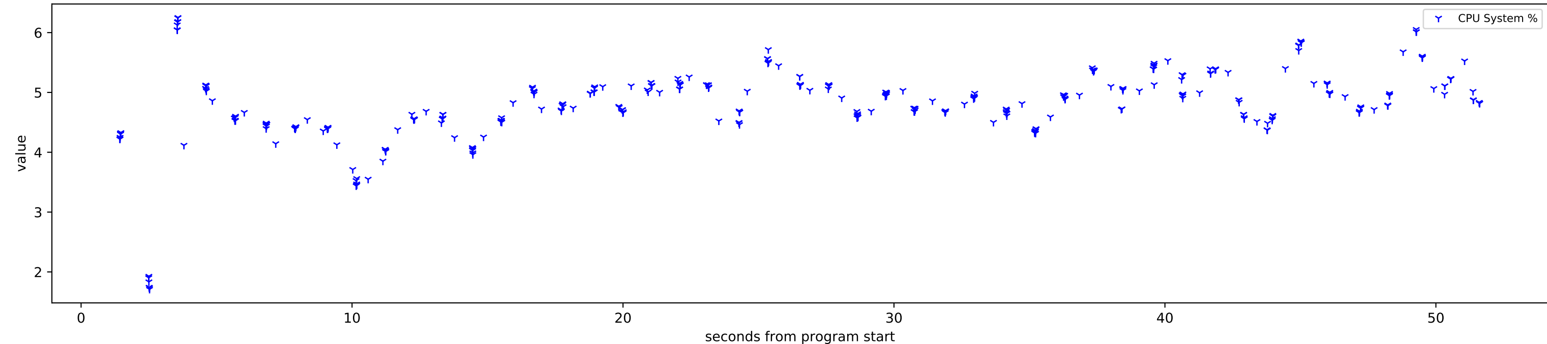
CPU System %
