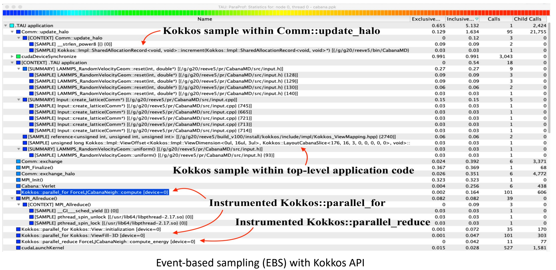
Event-based sampling (EBS) with Kokkos API
