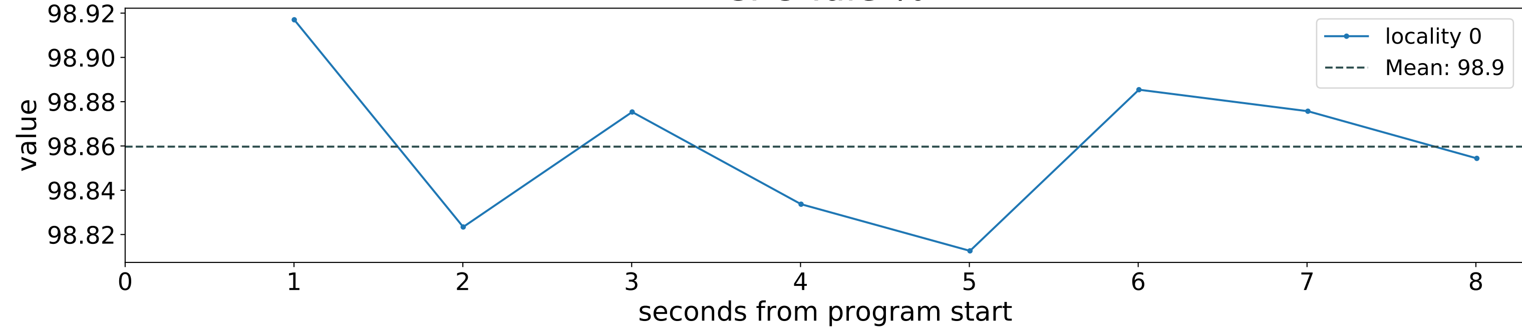
CPU Idle %
