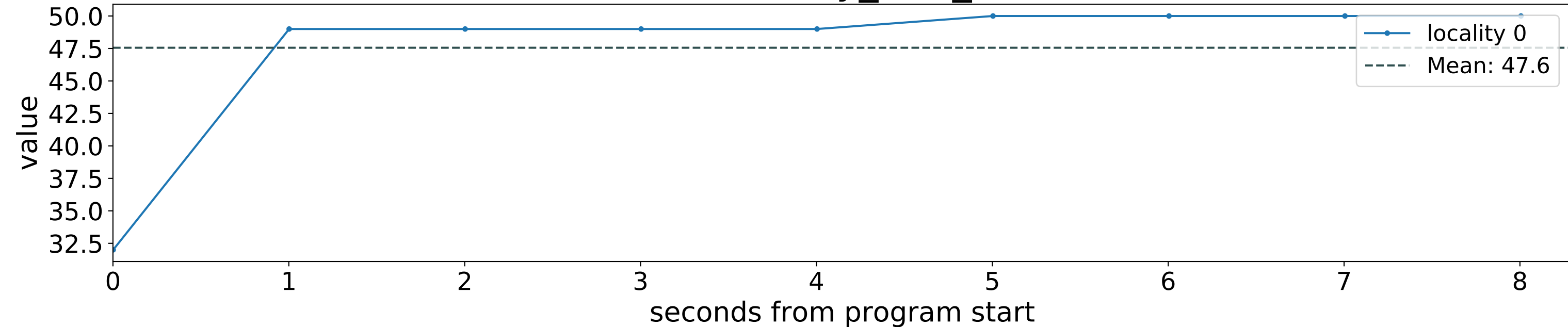
status:voluntary_ctxt_switches
