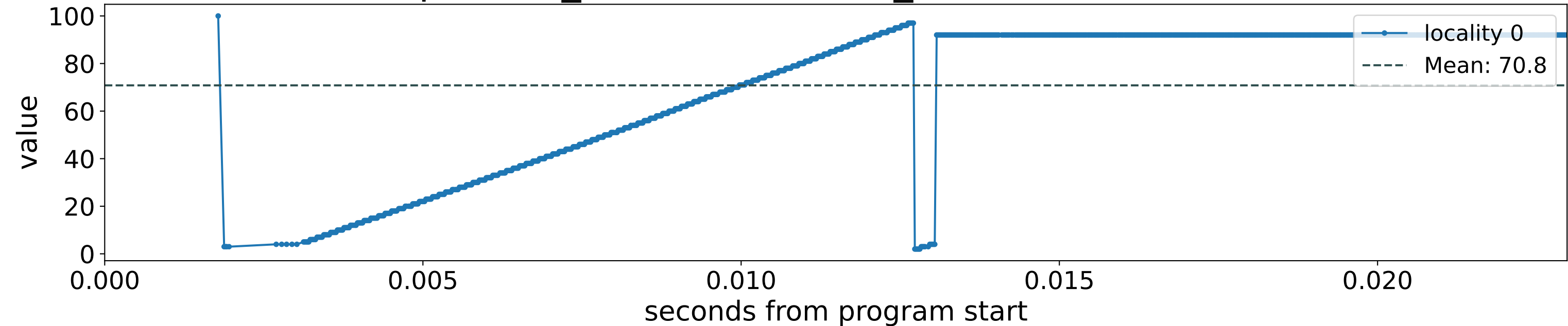
[2:parallel_for,1:Bench,tree_node:default]:Bench
