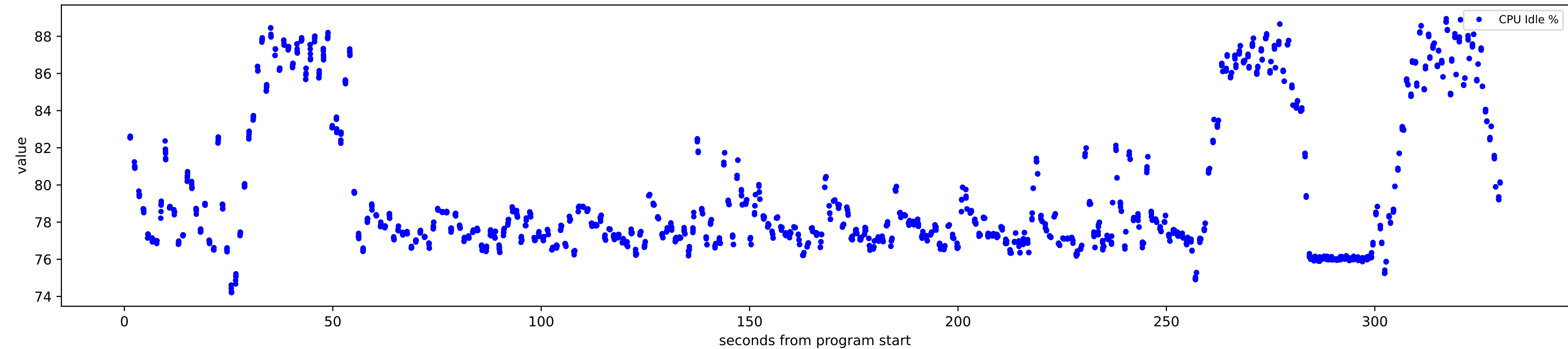
CPU Idle %
