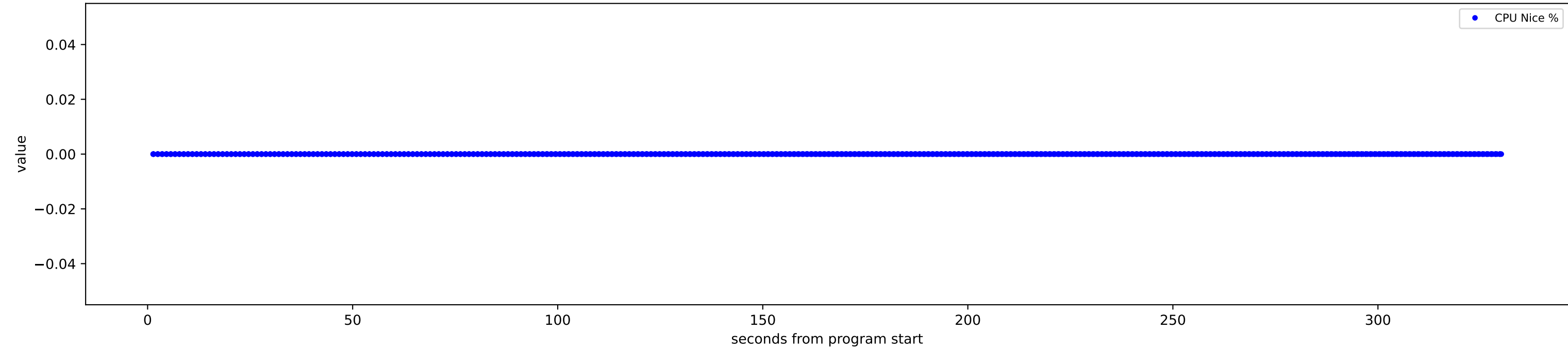
CPU Nice %
