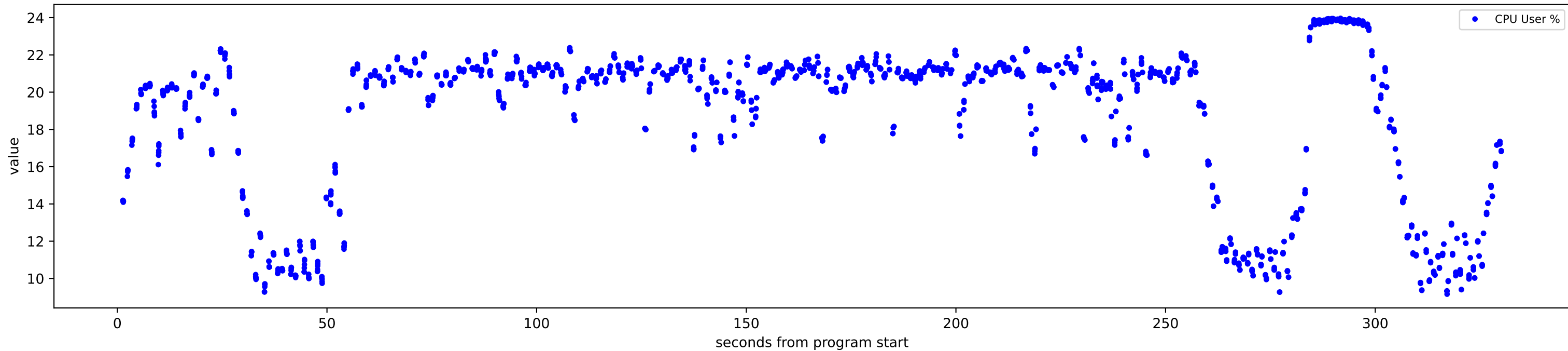
CPU User %
