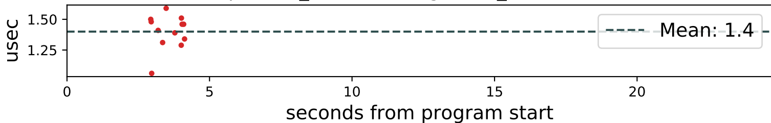
[2:parallel_for,1:MDRange,tree_node:default]
